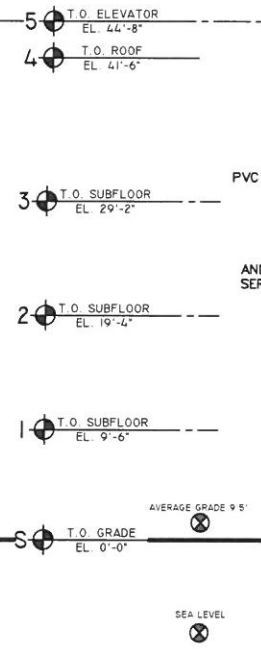
4 SOUTH ELEVATION SCALE: 1/16" = 1'-0"
