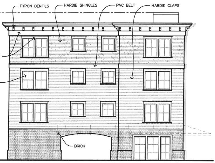
4 SOUTH ELEVATION SCALE: 1/16" = 1'-0"
